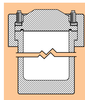
Cross Section 4671-4674
